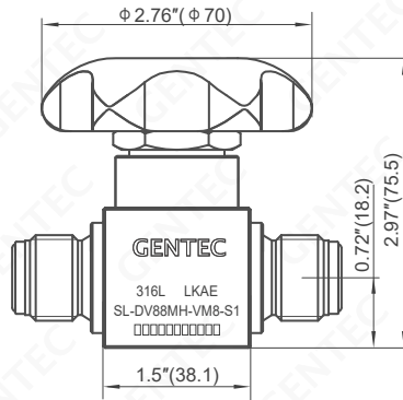
Handwheel (3500 psi)
