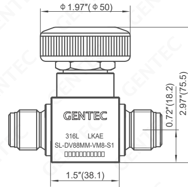
Handwheel (1500 psi)
