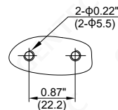
Rear Bracket Mounting
