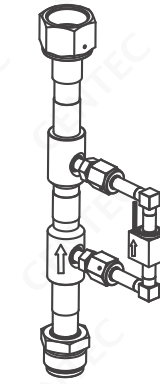
UFS20 Vertical Assembly
