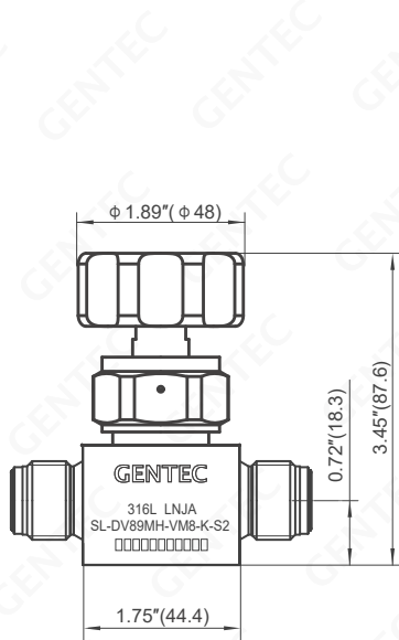
Handwheel
