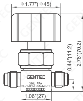
Handwheel (3500 psi)
