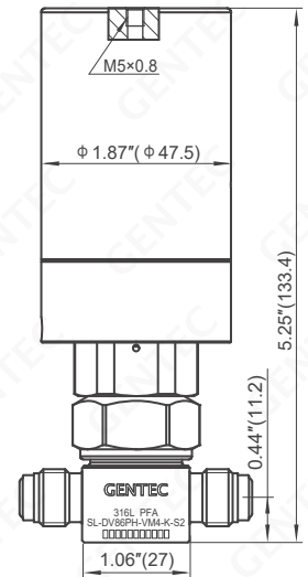
Pneumatic (3500 psi)
