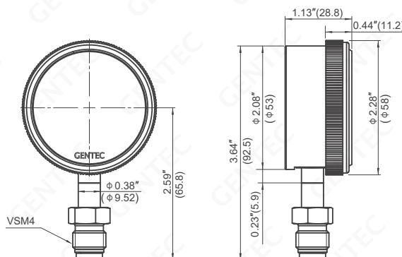
GU20SL-*-VSM4
